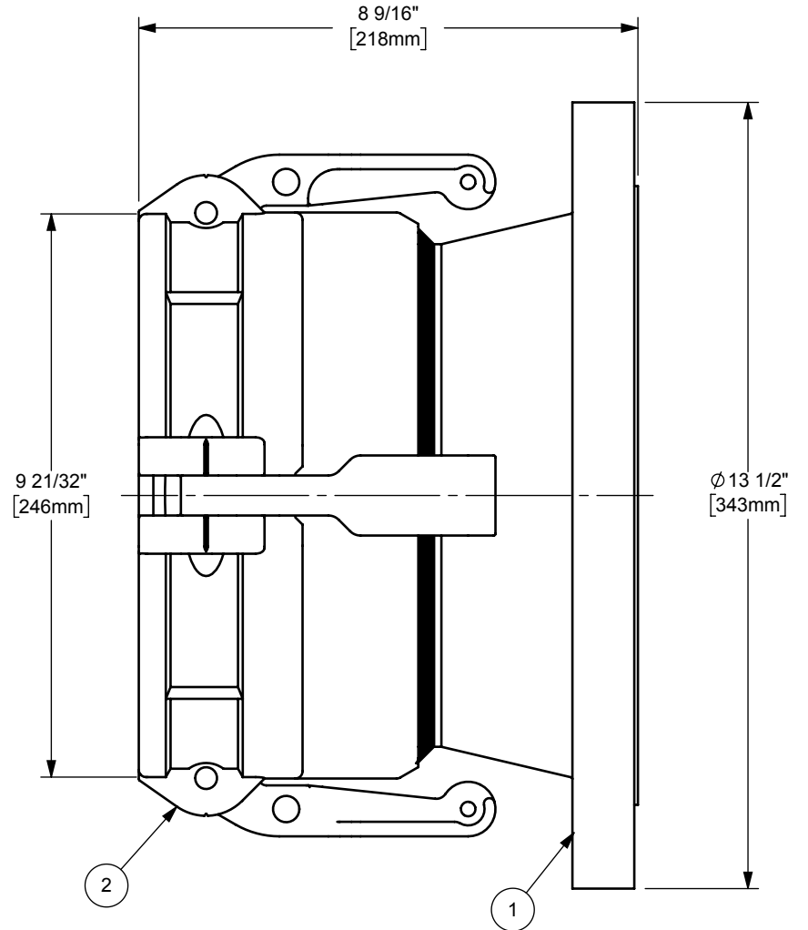
DIXON COUPLER USED AS REPRESENTATION OF PT COUPLER
